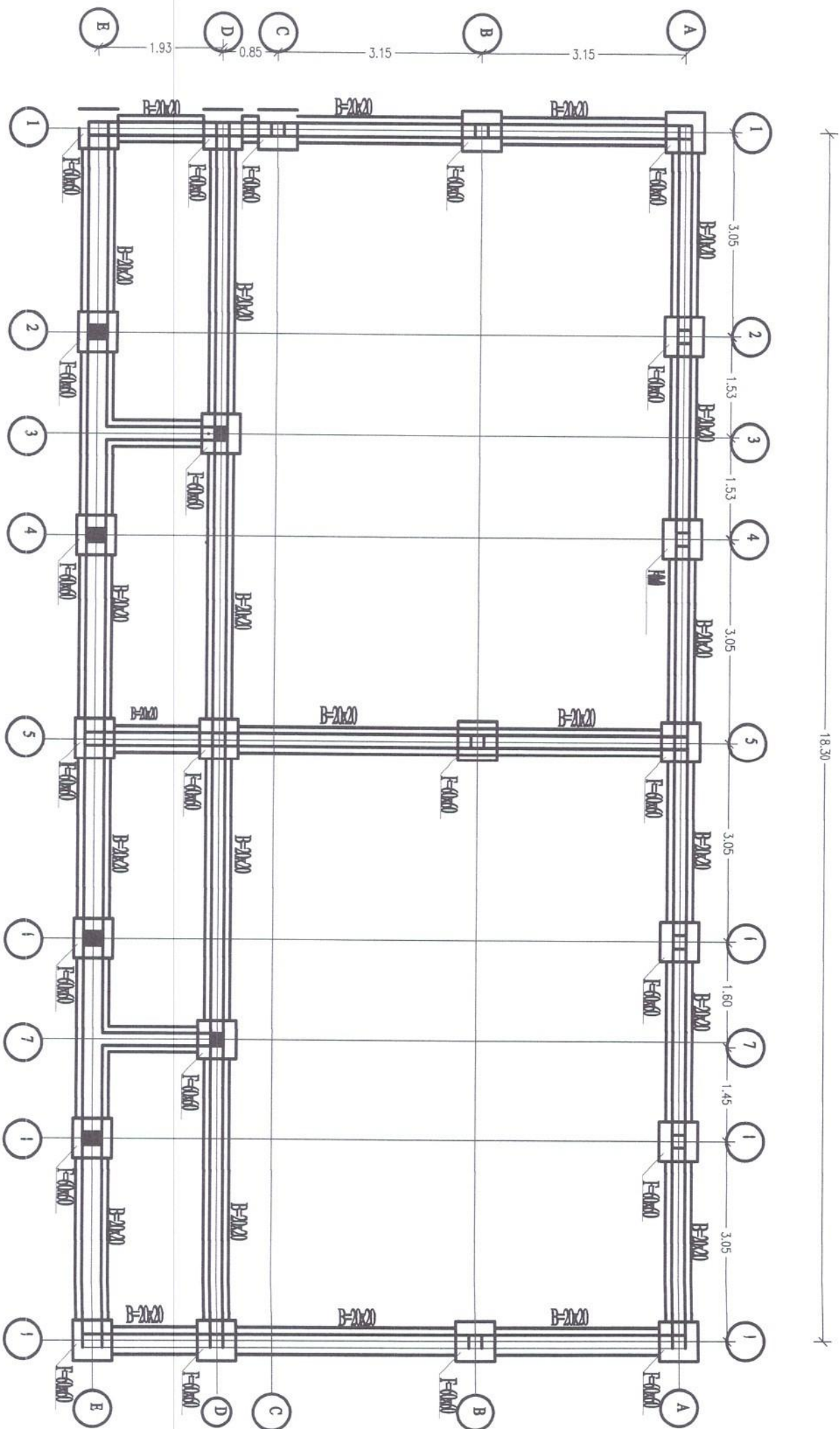
FOUNDATION PLAN
